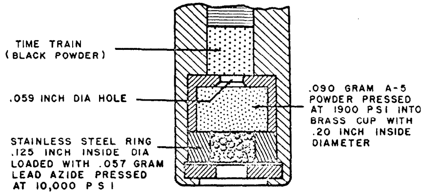
Fig 1-64 RELAY DETONATOR
